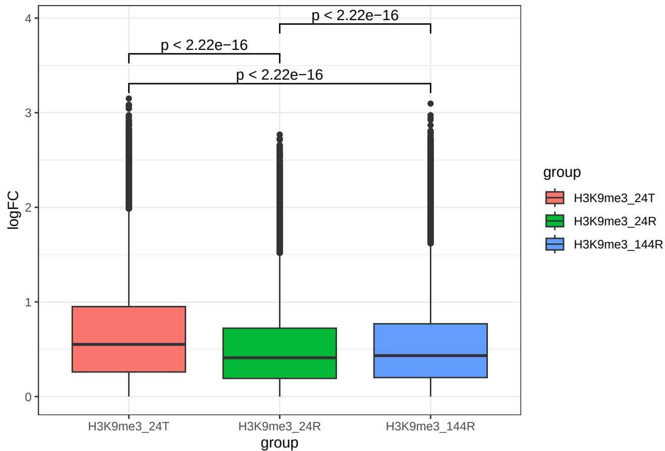
Absolute LFC across time for H3K9me3 set1
